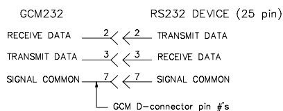
TYPICAL RS232 CONNECTIONS
