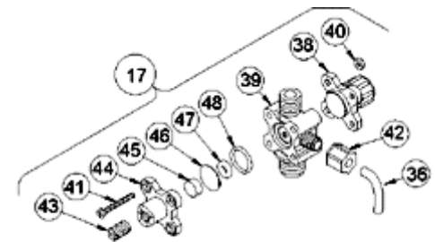
4-FUNCTION BLEED VALVE (B-4FV)
