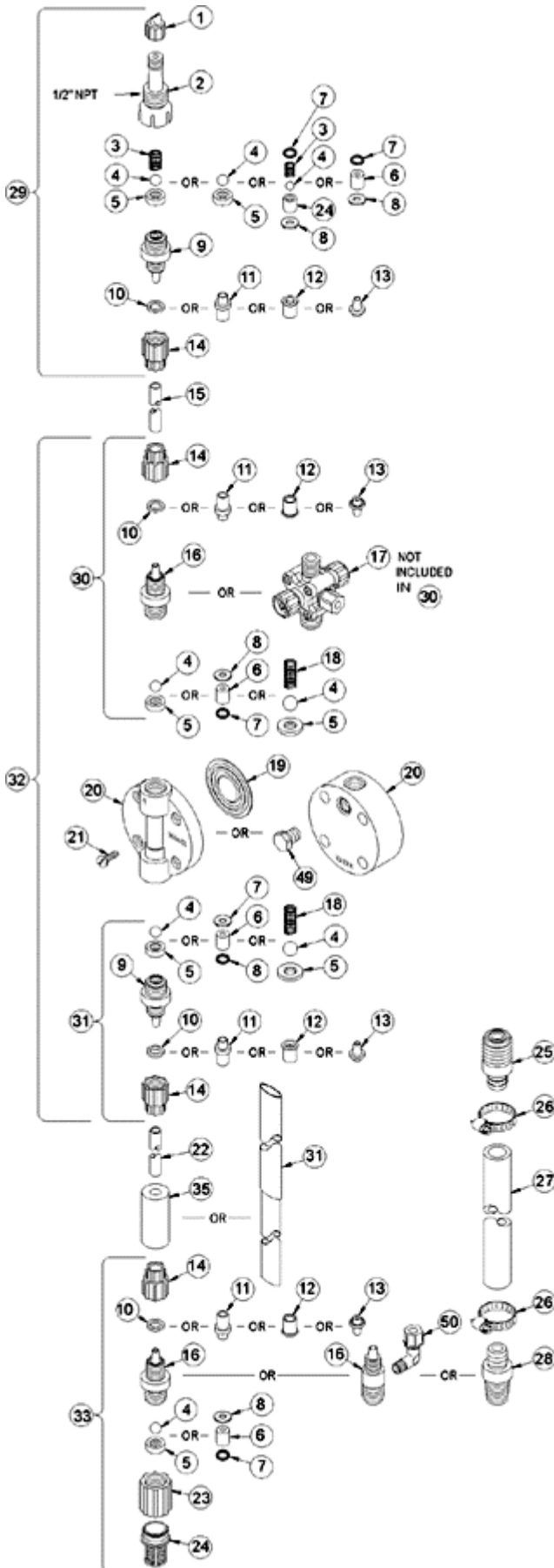
4-FUNCTION BLEED VALVE (B-4FV)
