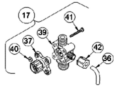
3-FUNCTION VALVE (3FV)
